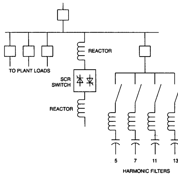
Figure 8-7—Static var control
