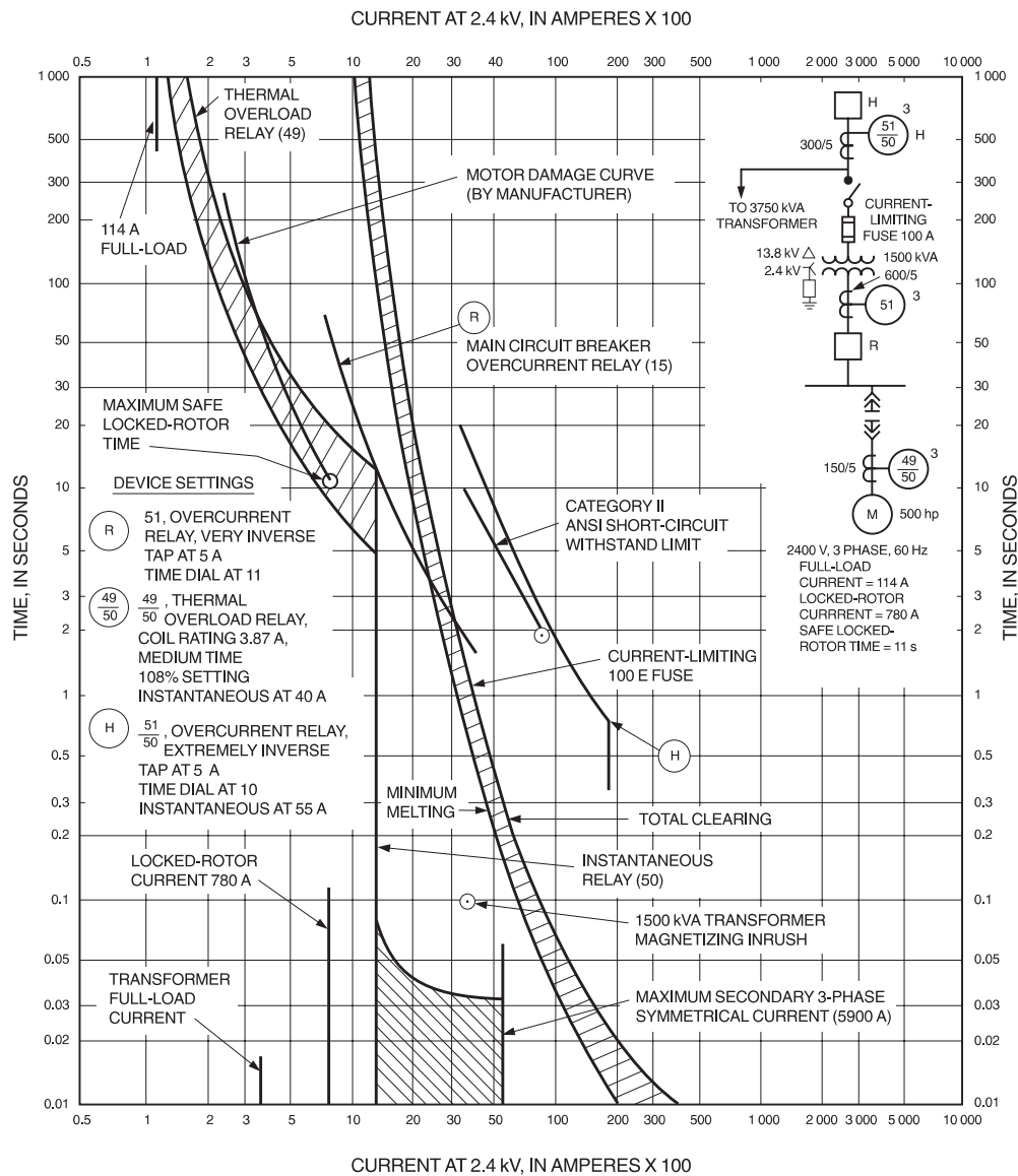
Figure 5-34—Phase-relay time-current characteristic curves for 2.4 kV Bus 1 coordination
