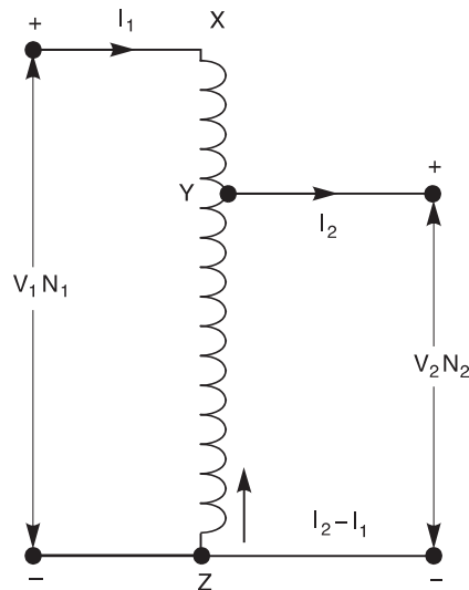
Figure 10-1—Typical autotransformer
