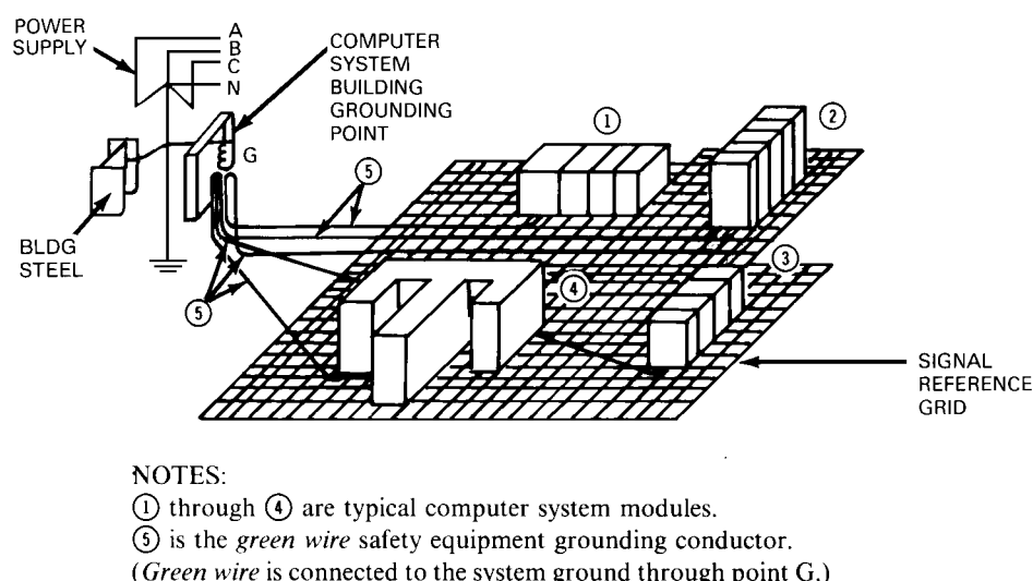
Figure 7-5—Computer units connected to signal reference grid and to ac ground
