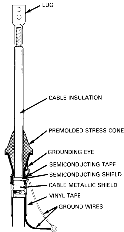
Figure 12-12—Typical Class 3 rubber terminator (for solid dielectric cable)
