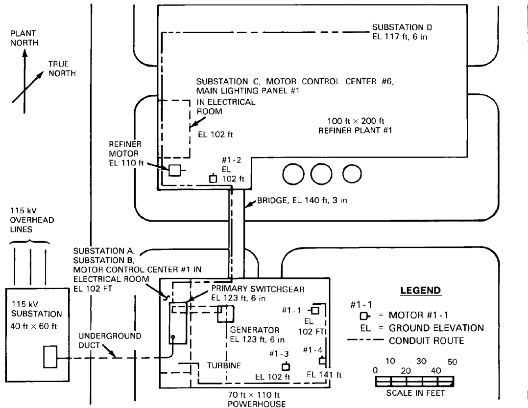
Figure 16-4—Site plan
