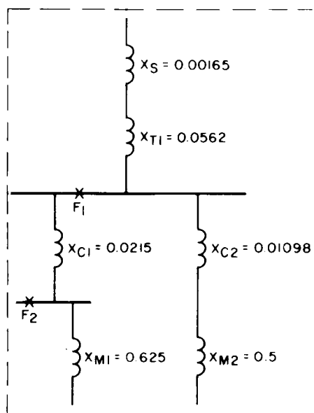
Figure 4-22—Reactance network for faults at F_1 and F_2
