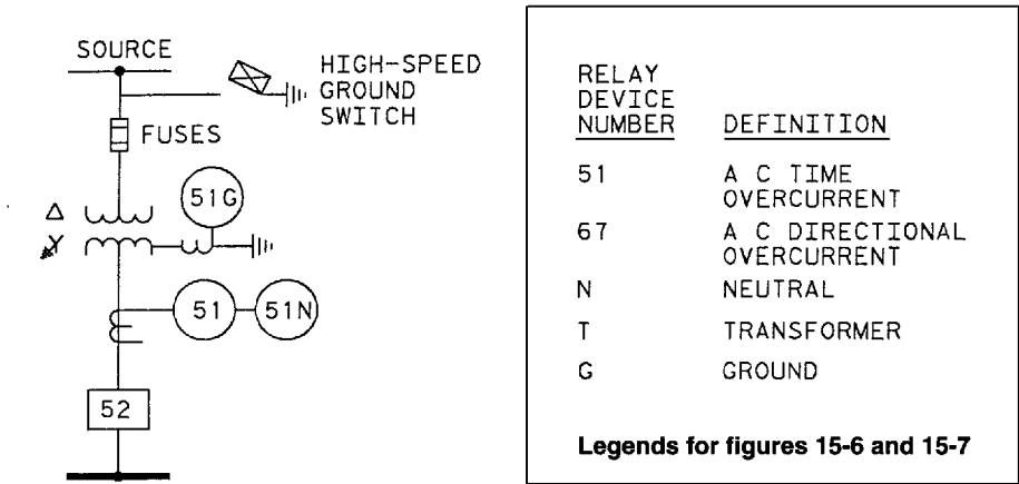
Figure 15-6—Transformer protection with primary fuses (no load or metering circuits shown)
