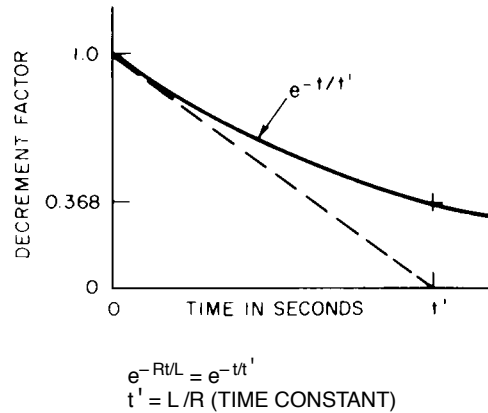
Figure 4-5—Decrement factor
