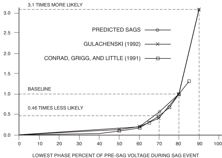
Figure 3-9—Voltage sag probabilities
