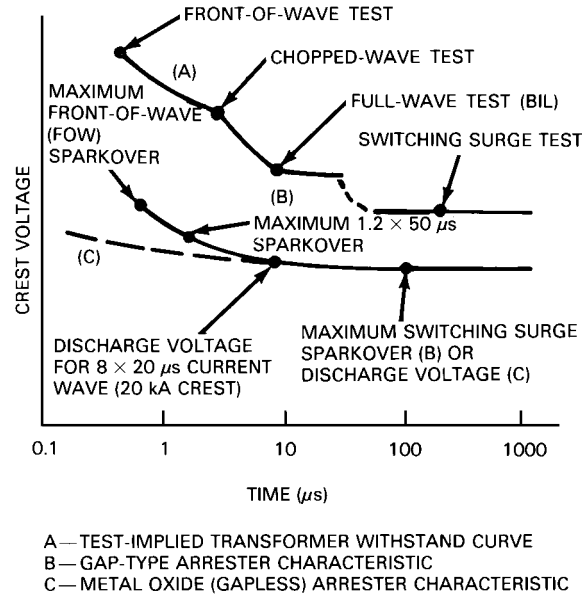
Figure 6-16—Insulation coordination based on test-implied transformer withstand curve
