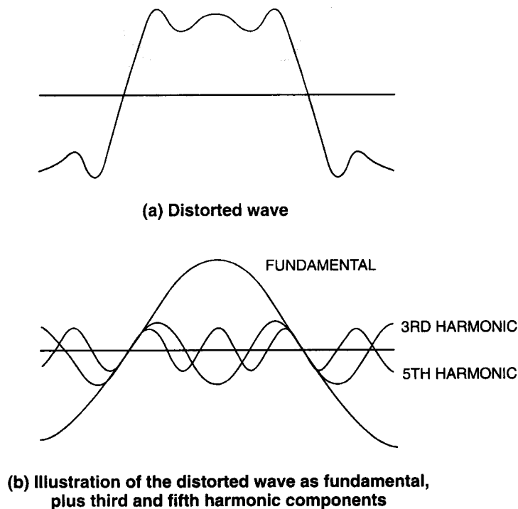
Figure 9-2—Decomposition of a distorted wave
