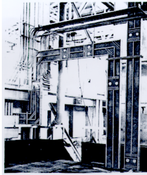
Figure 13-3—Feeder busway
