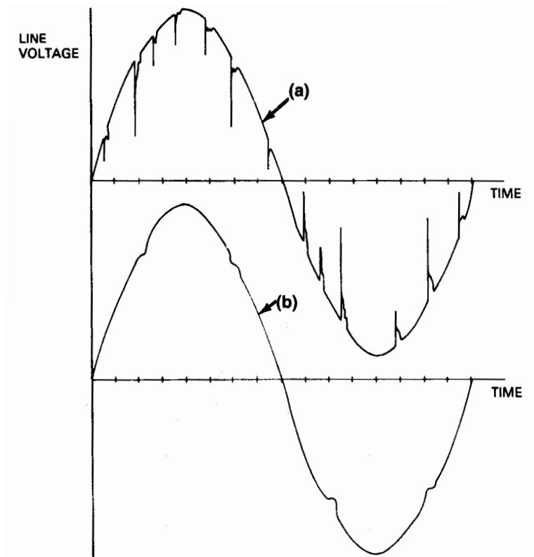
Figure 8-21—Illustration of the reduction of rectifier commutation switching transients by the application of power capacitors
