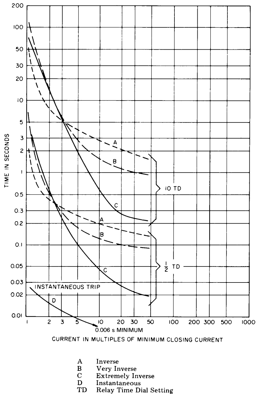
Figure 5-7—Typical relay time-current characteristics
