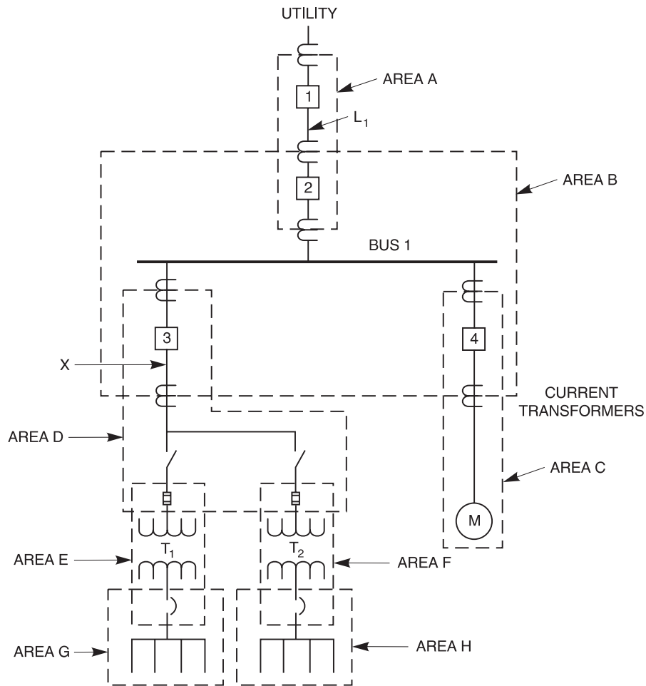
Figure 5-16—One-line diagram illustrating zones of protection
