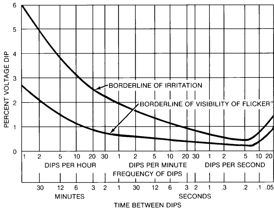
Figure 3-8—Range of observable and objectionable voltage flicker versus time
