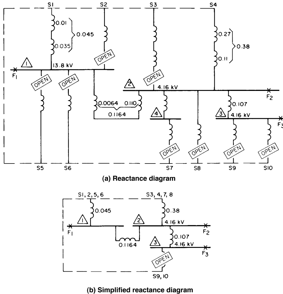
Figure 4-19—Circuits of power system reactances for calculation of approximately 30-cycle minimum short-circuit currents
