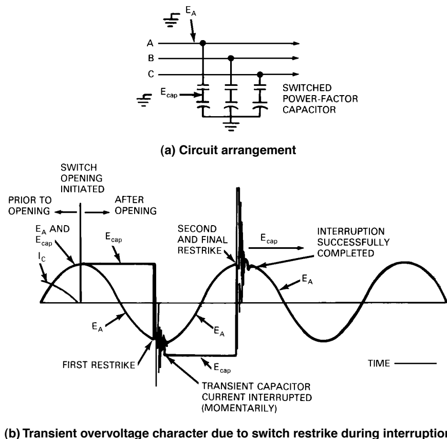
Figure 6-3—Equivalent circuit and transient response for capacitor switching restrike phenomena
